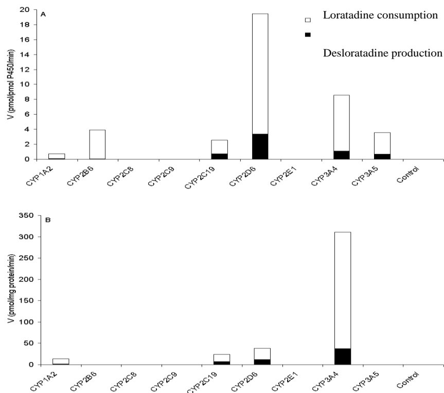
Figure 1. Comparison between the amount of desloratadine produced and the amount of loratadine consumed over 30 min incubation of loratadine with different CYP, before (A) and following (B) the RAF method.
