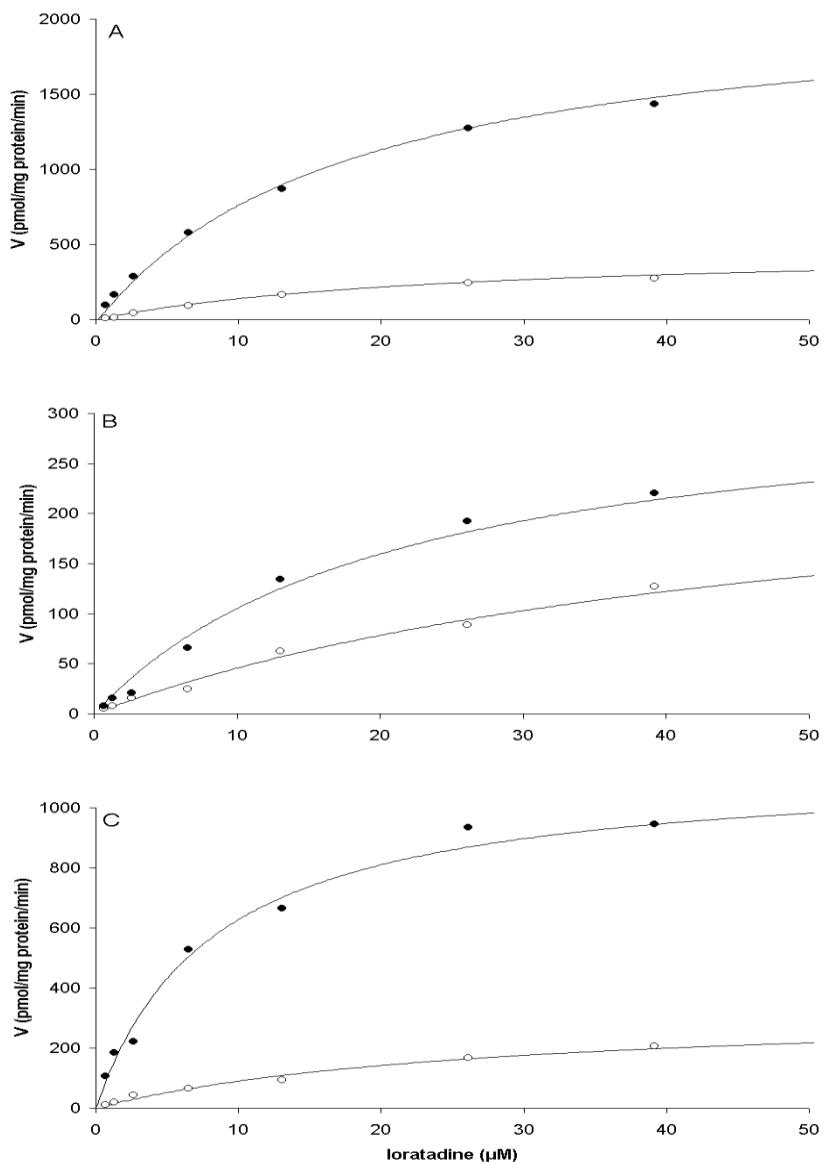
Figure 2. Enzymatic kinetic modelling of loratadine disappearance (solid circles), and desloratadine formation (empty circles) with human liver microsomes (A), CYP 2D6 (B) and CYP 3A4 (C) Supersomes using the Michaelis-Menten function. (A and B) results are presented as the mean of duplicates obtained with recombinant CYP and scaled to HLM following the RAF method.
