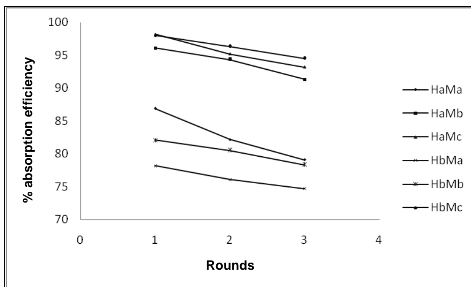
Figure 7. Absorption-desorption rounds of PHEMA magnetic nanogels.
